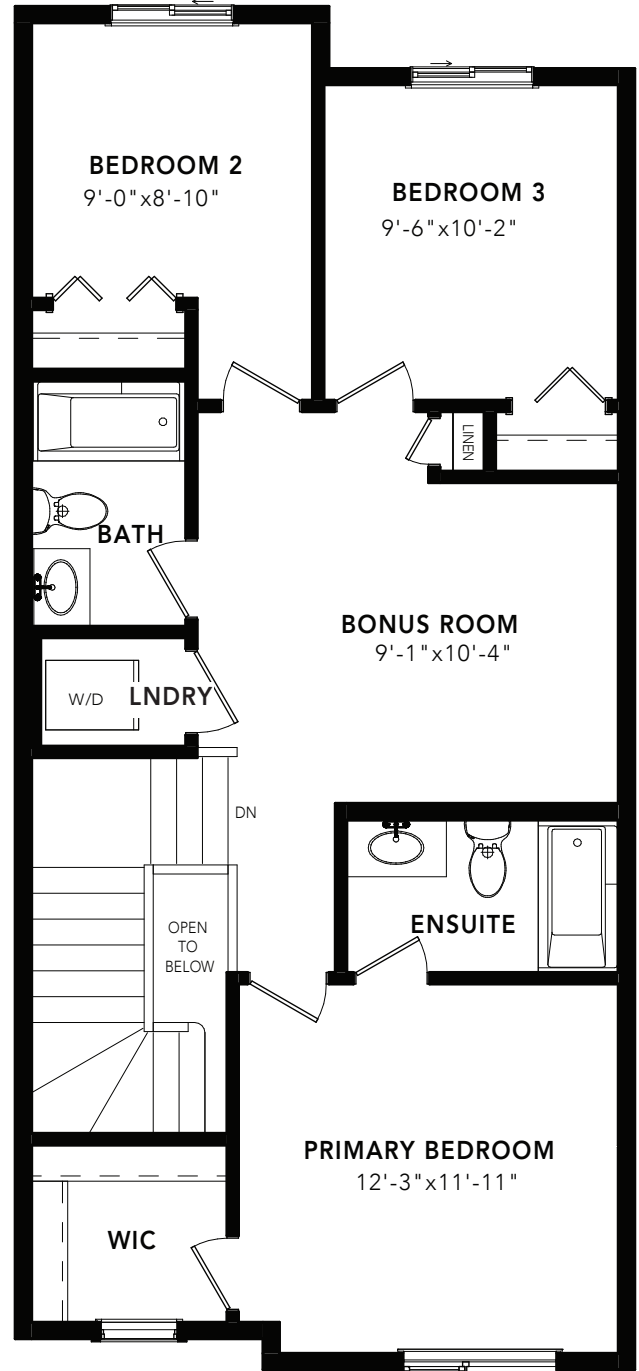
SECOND FLOOR: 841 SQ FT
