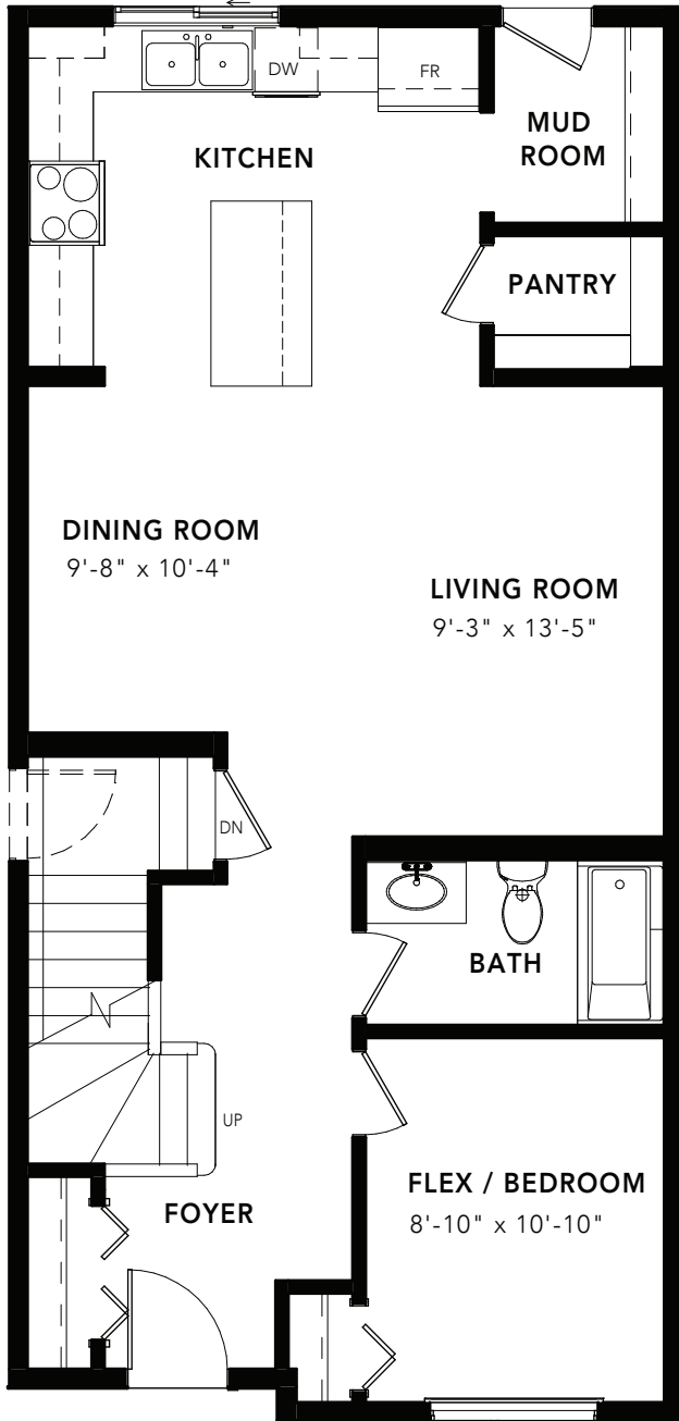
MAIN FLOOR : 832 SQ FT
