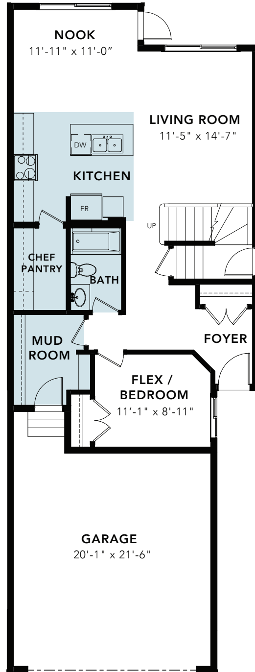
CHEF PANTRY & FULL BATH OPTION: 942 SQ FT
