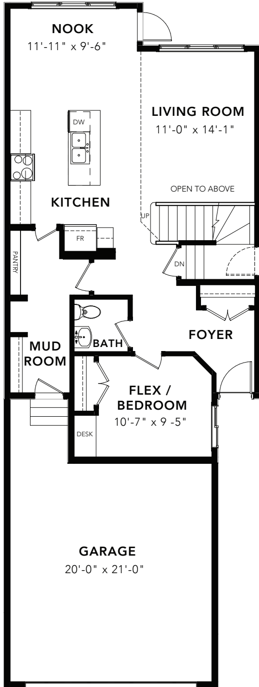
MAIN FLOOR : 928 SQ FT
