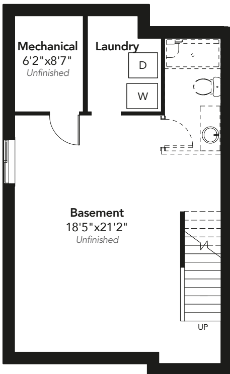
BASEMENT 540 SQ FT
