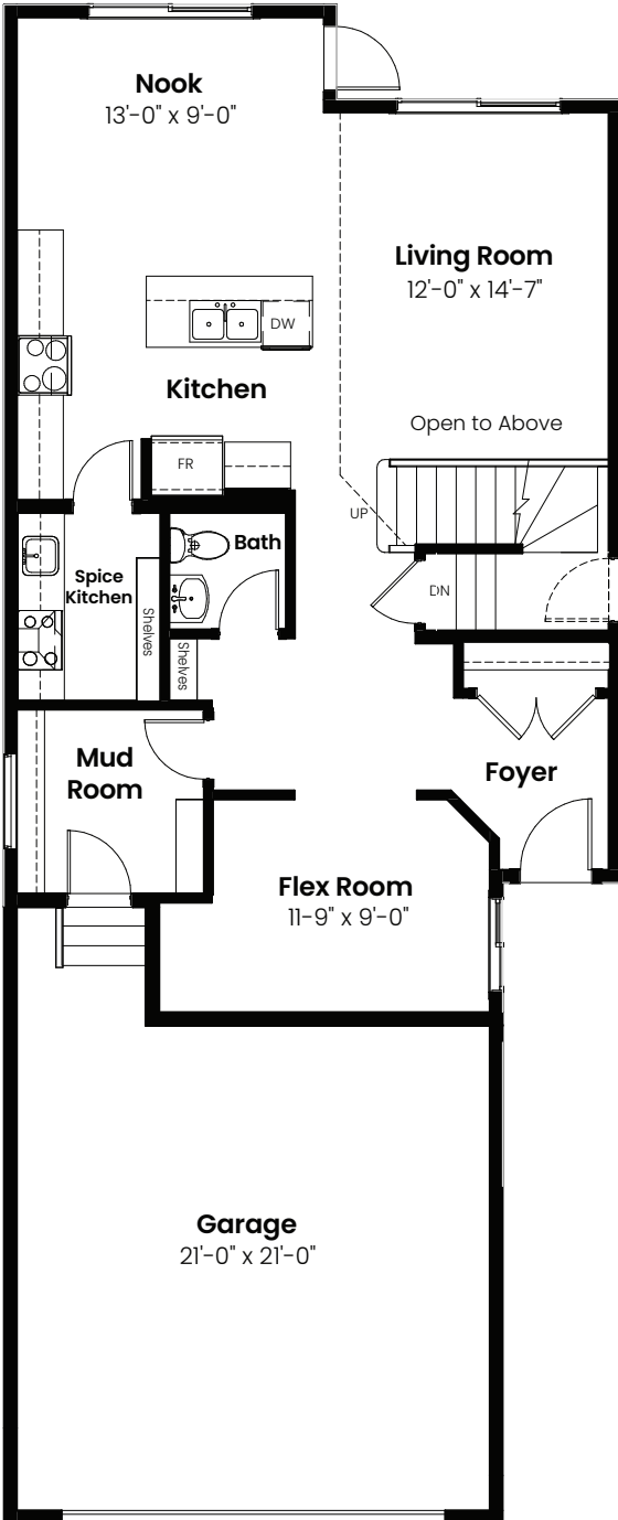
Spice Kitchen Option: 1010 Sq Ft
