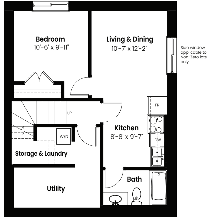
Basement Suite Option: 481 Sq Ft
