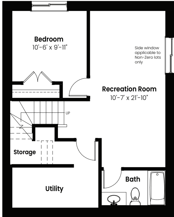
Basement Development Option: 481 Sq Ft
